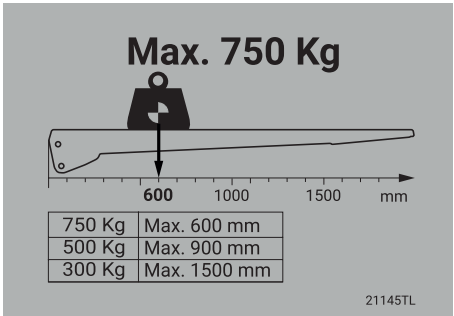
Loading diagram
