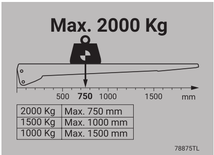
Loading diagram
