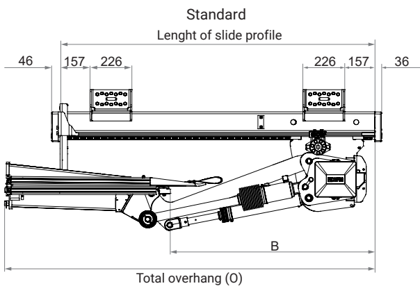
Installation dimensions (mm)
