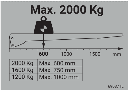
Loading diagram
