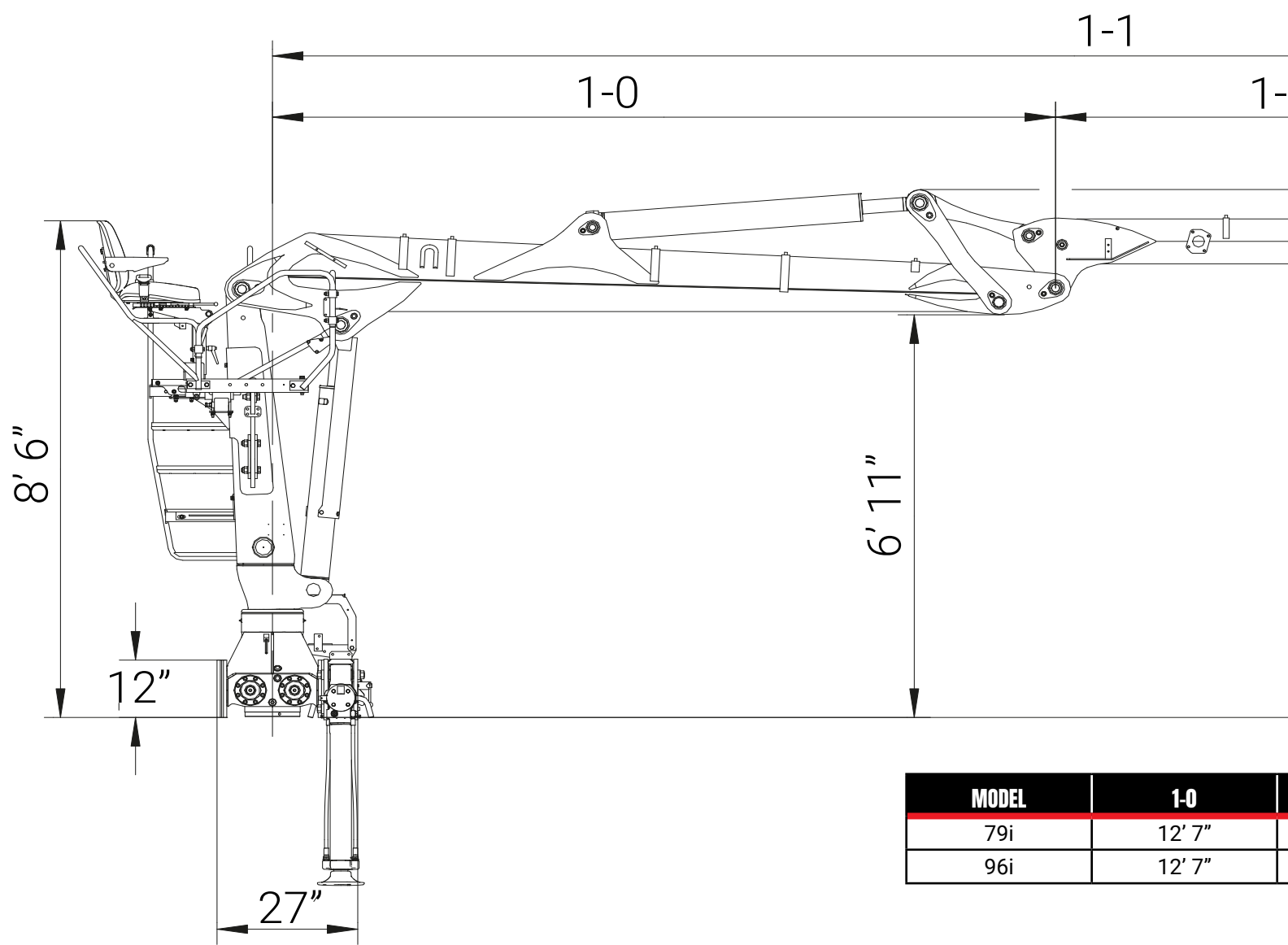
Side View
