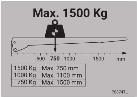
Loading diagram
