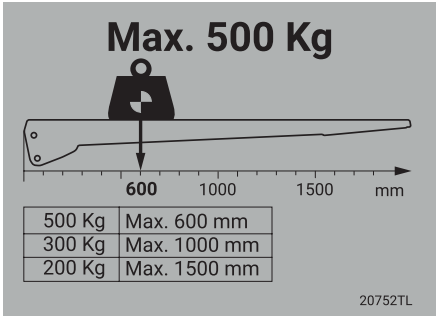
Loading diagram
