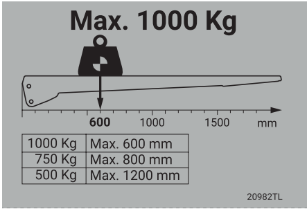
Loading diagram
