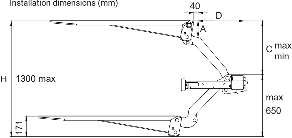
Installation dimensions (mm)
