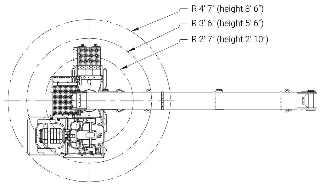
Slewing radius
