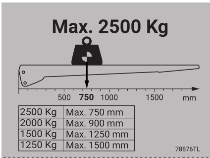
Loading diagram
